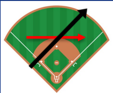
FRI Winds
