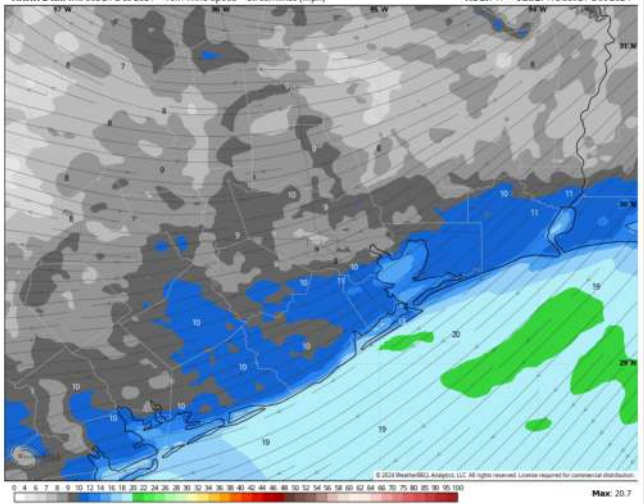
HRRR 3 km Init 00z 21 Dec 2024 • 10m Wind Speed • Streamlines (mph) Hour: 17 • Valid: 17z Sat 21 Dec 2024
