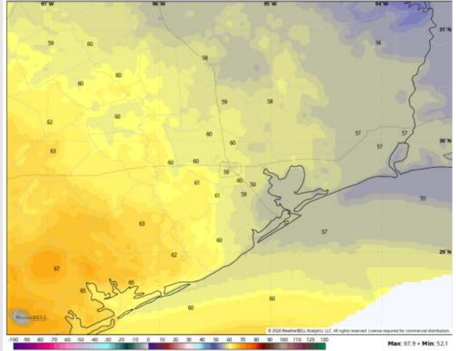
NDFD 2.5 km Init 04z 21 Dec 2024 • Daily Max. 2m Temperature (°F) Valid: Sat 21 Dec 2024
