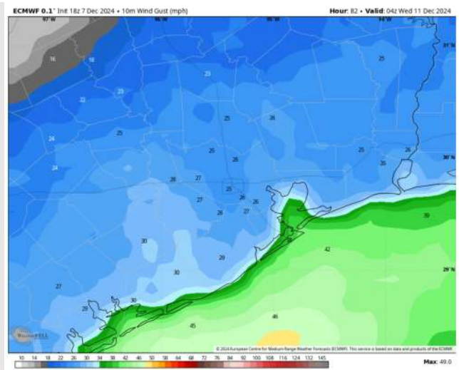
Wind Gusts 10 PM CT
