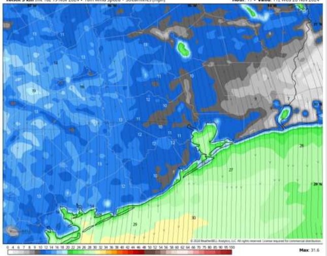
HRRR 3 km Init 18z 19 Nov 2024 • 10m Wind Speed • Streamlines (mph) Hour: 17 • Valid: 11z Wed 20 Nov 2024
