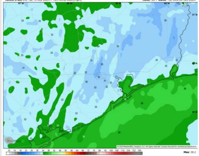
HRRR 3 km Init 18z 19 Nov 2024 • 10m Wind Gust (mph) Hour: 22 • Valid: 16z Wed 20 Nov 2024
