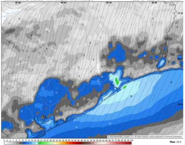
HRRR 3 km Init 12z 13 Oct 2024 • 10m Wind Speed + Streamlines (mph) Hour: 12 • Valid: 00z Mon 14 Oct 2024
