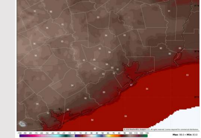
NDFD 2.5 km Init 03z 17 Sep 2024 • Daily Max, 2m Temperature (°F) Valid: Wed 18 Sep 2024
