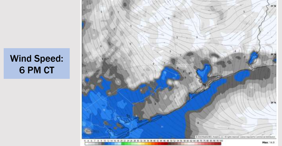
HRRR 3 km Init 00z 17 Sep 2024 • 10m Wind Speed • Streamlines (mph) Hour: 47 • Valid: 23z Wed 18 Sep 2024
