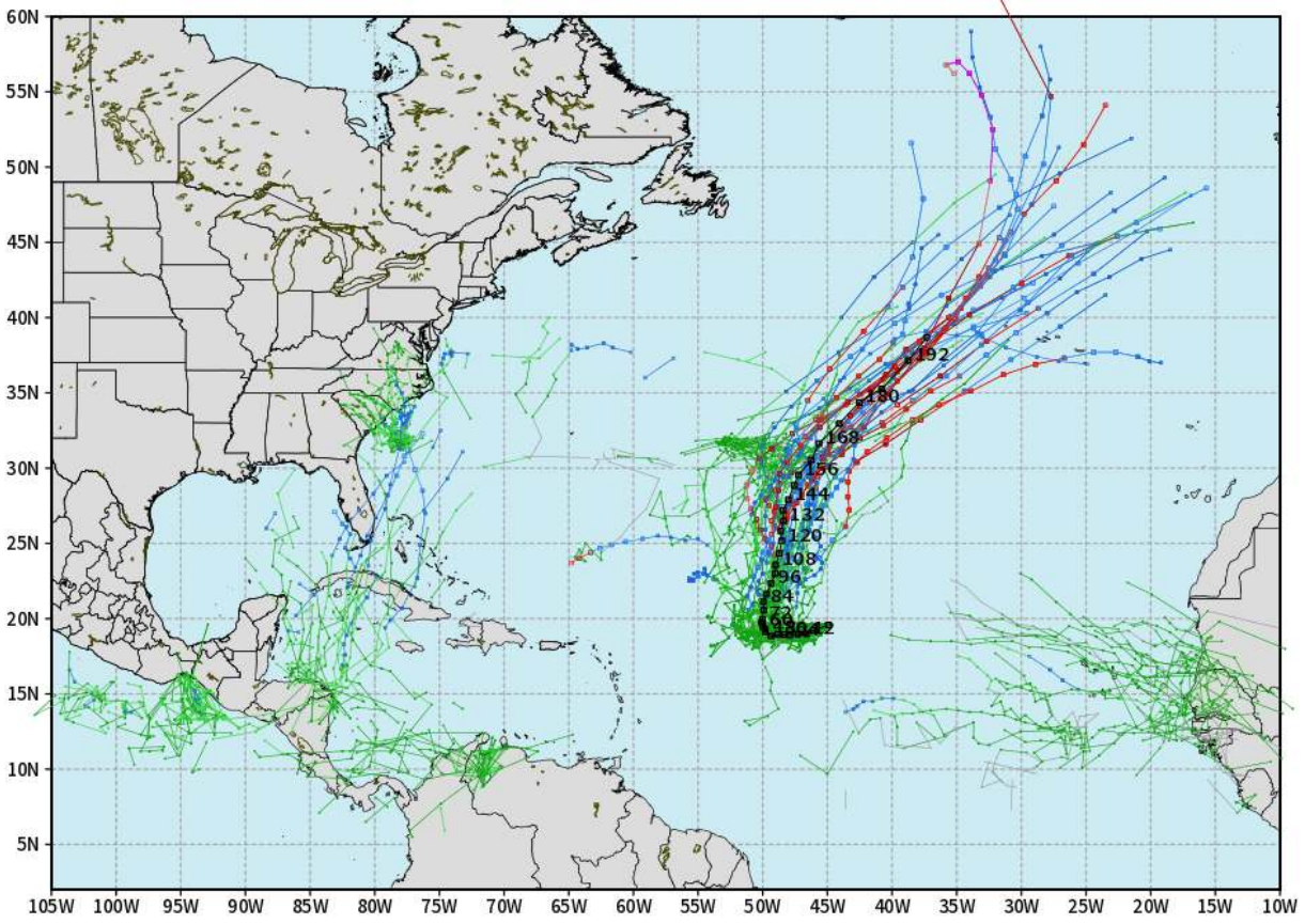
ECMWF ATLANTIC EPS Cyclone Locations --> Next [10-days] INIT: 12Z15SEP2024 --> UNTIL 12Z25SEP2024
