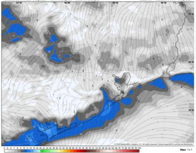
HRRR 3 km Init 00z 16 Sep 2024 • 10m Wind Speed • Streamlines (mph) Hour: 21 • Valid: 21z Mon 16 Sep 2024
