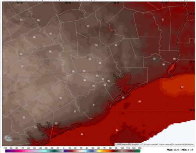
NDFD 2.5 km Init 01z 16 Sep 2024 • Daily Max: 2m Temperature (°F) Valid: Mon 16 Sep 2024
