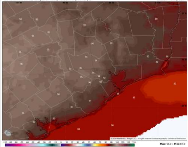
NDFD 2.5 km Init 17z 12 Sep 2024 • Daily Max: 2m Temperature (°F) Valid: Fri 13 Sep 2024
