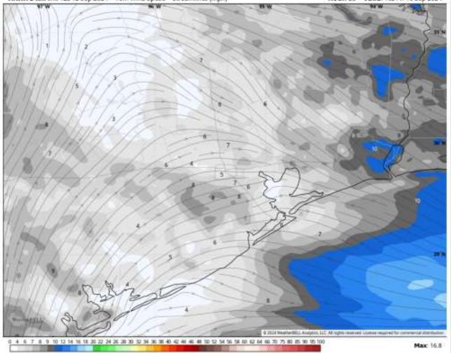
HRRR 3 km Init 12z 12 Sep 2024 • 10m Wind Speed • Streamlines (mph) Hour: 28 • Valid: 16z Fri 13 Sep 2024
