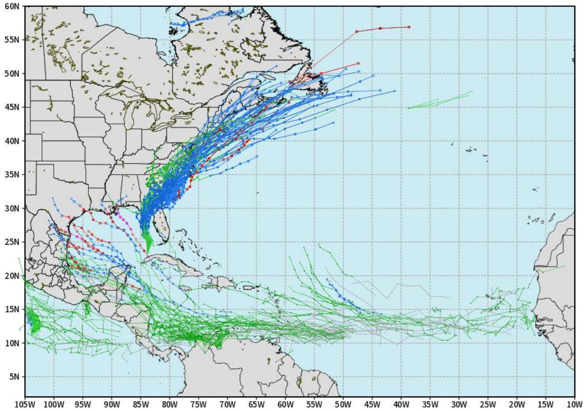
ECMWF ATLANTIC EPS Cyclone Locations --> Next [10-days] INIT: 00Z04AUG2024 --> UNTIL 00Z14AUG2024
