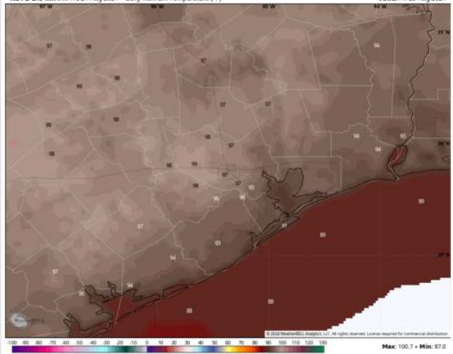
NDFD 2.5 km Init 17z 21 Aug 2024 • Daily Max, 2m Temperature (°F) Valid: Fri 23 Aug 2024
