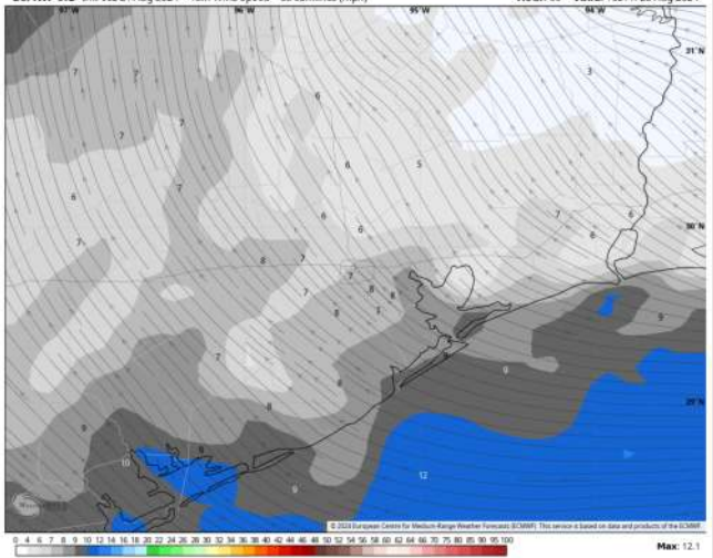
ECMWF 0.1° Init 06z 21 Aug 2024 • 10m Wind Speed • Streamlines (mph) Hour: 60 • Valid: 18z Fri 23 Aug 2024
