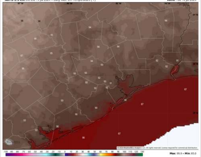
NDFD 2.5 km Init 03z 15 Jul 2024 • Daily Max 2m Temperature (F) Valid: Tue 16 Jul 2024
