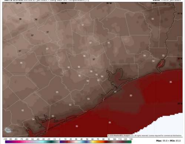
NDFD 2.5 km Init 03z 27 Jun 2024 • Daily Max, 2m Temperature (°F) Valid: Thu 27 Jun 2024
