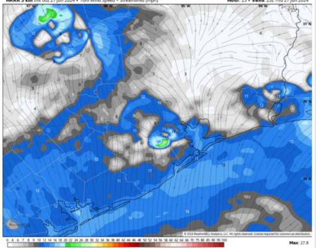
HRRR 3 km Init 00z 27 Jun 2024 • 10m Wind Speed • Streamlines (mph) Hour: 23 • Valid: 23z Thu 27 Jun 2024
