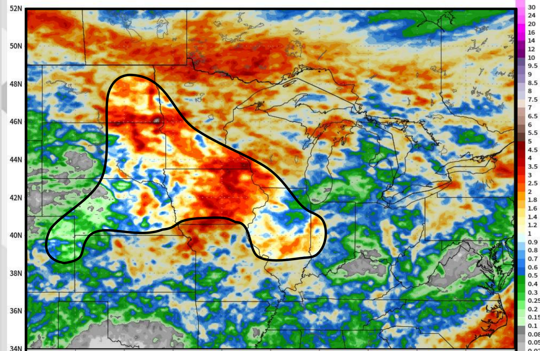
ECMWF 7-DAYS Precipitation [inch] b/t 12Z27JUN2024 -- 12Z04JUL2024 Init: 12Z27JUN2024 -- [168] hr --> Valid Thu 12Z04JUL2024
