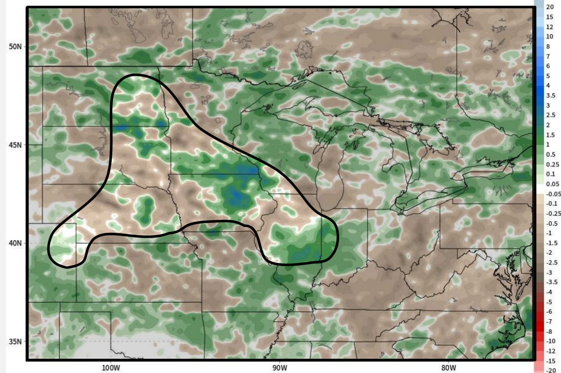
ECMWF HRES Total Precipitation [inches] | Days 0 to 7 | Model Cycle Difference [CURRENT minus 12-h PRIOR] Init: 12Z27JUN2024 -- [168] hr --> Valid Thu 12Z04JUL2024
