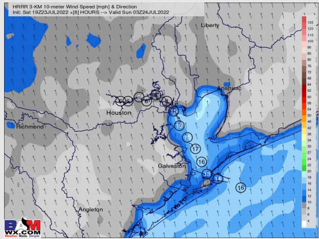
Wind Speed 10 PM CT
