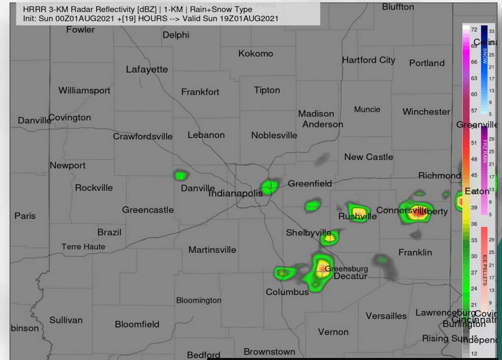
Sunday 3PM Simulated Radar
